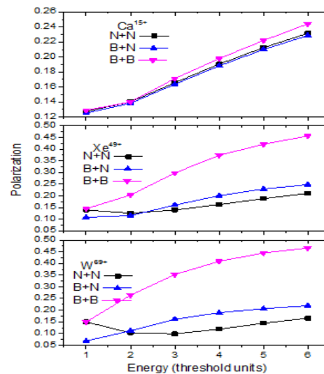
Figure 1. The linear polarization of the transition 1s to 2p of \text{Ca}^{15+} , \text{Xe}^{49+} and \text{W}^{69+} ions. N+N represents without Breit interaction in calculations of the target wave functions and impact matrix element, B+N represents with Breit interaction in calculations of the target wave functions and without Breit interaction in calculations of the impact matrix element, B+B represents with Breit interaction in calculations of the target wave functions and impact matrix element.
