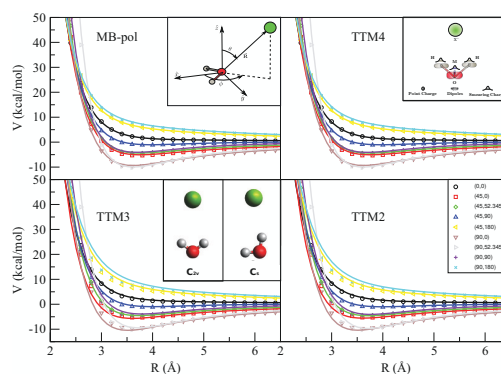
Figure 1. Potential curves (solid lines) and corresponding CCSD(T)-F12 reference data (symbols) calculated for different (\theta, \phi) orientations of the I^- (H_2O) dimers employing the indicated TTM water models. In the insert panels we display the coordinate system used (upper/left), the charge and dipole-moment positions for i-TTM4/MB-pol models (upper/right), and the C_s and C_{2v} minimum and saddle-point geometries of I^- (H_2O) (lower/left).
