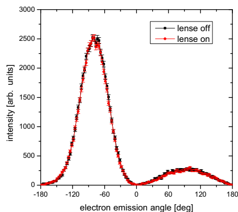
Figure 1. Electron emission angle in the scattering plane for 2 MeV p+He, E_e=6.5\pm3.5 eV, q=0.75\pm0.25 au, with projectile lense turned on (red circles) or turned off (black squares).
