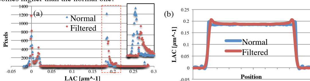
Fig. 5: (a) Histograms of the CT image of the normal and Gaussian filtered phantoms and inset shows detail of the peak around 0.185 \mu\text{m}^{-1} , (b) profiles of reconstructed images
