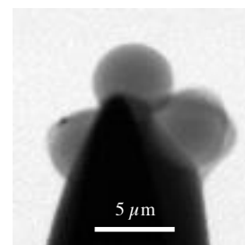
Fig. 2: STXM image of a sample
