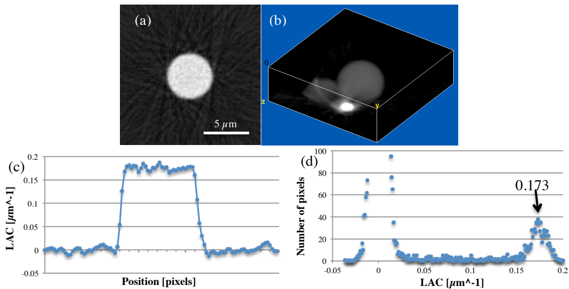
Fig. 3: Reconstructed images of the polystyrene spheres; (a) a cross sectional image and (b) 3-dimensional volume image. (c) A profile along radial direction and (d) a histogram of (a).
