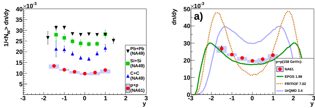
Figure 3. (left) Rapidity distribution of \Lambda hyperons divided by the number of wounded nucleons in inelastic p+p interactions at 158 GeV/c together with the data from Si+Si, C+C [8], and Pb+Pb [9] collisions; (right) comparison of the \Lambda rapidity distribution in p+p collisions to calculations by the EPOS [10], UrQMD [11, 12], and Fritiof [13] models.
