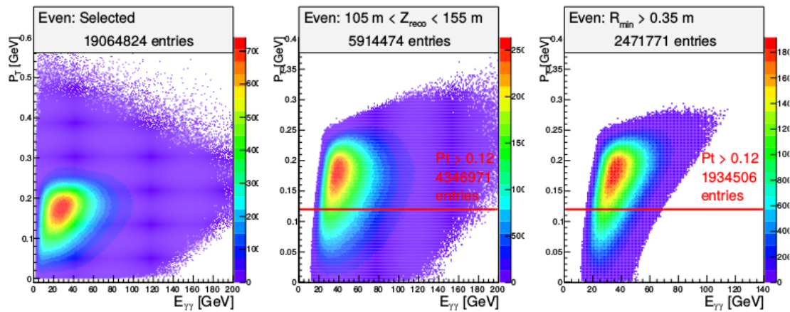
Figure 4. Transverse momentum vs 2-photon energy ( p_{\perp} vs E_{\gamma\gamma} ) for simulated signal events with (left) both photons on the LKr, (center) vertex reconstructed within fiducial volume, and (right) r > 35\text{ cm} for both LKr clusters. The p_{\perp} > 0.12\text{ GeV}/c boundary is overlaid center and right. Note scale changes between plots.
