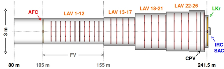
Figure 2. Neutral detector layout: AFC = active final collimator, LAV = large-angle veto, FV = fiducial volume, CPV = charged-particle veto, LKr = liquid Krypton calorimeter, IRC = inner-ring calorimeter, SAC = small-angle calorimeter.
