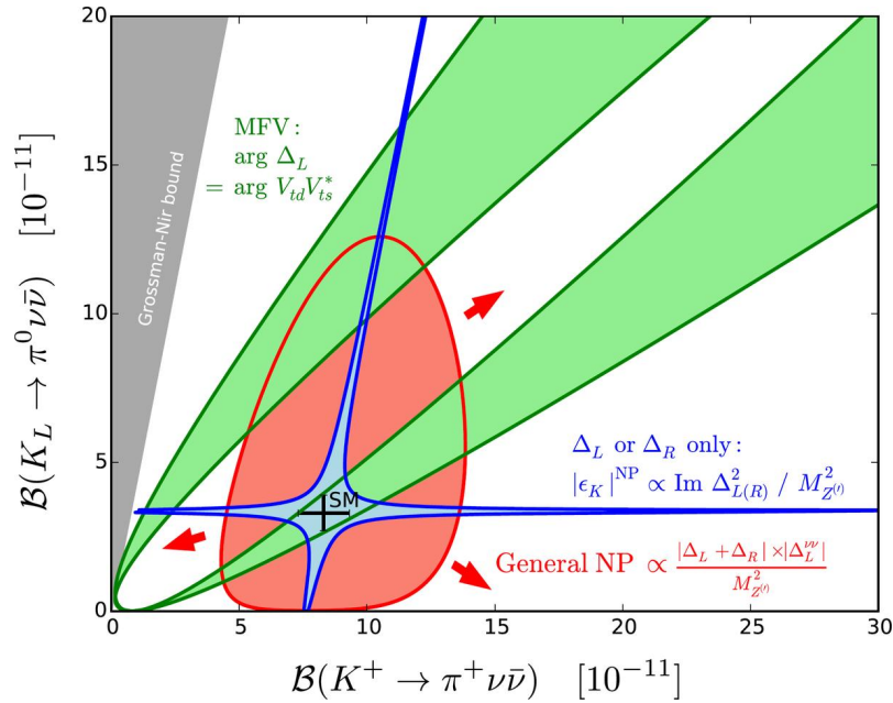
Figure 1. Sensitivity to new physics (NP) [1]. Measurements of both branching ratios can in principle distinguish among different classes of NP models: (diagonal swaths) CKM-like flavor structure, such as minimal flavor violation; (cross-like structure) new flavor-violating interactions in which either LH or RH couplings dominate, such as Z/Z' or T-parity Higgs; (blob) Unconstrained flavor sectors, such as Randall-Sundrum.
