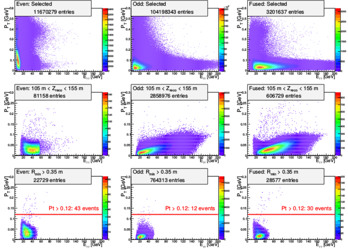
Figure 5. Transverse momentum vs 2-photon energy ( p_{\perp} vs E_{\gamma\gamma} ) for simulated K_L^0 \rightarrow \pi^0\pi^0 events. From left to right, the columns are even, odd, and fused events, respectively. The first row shows events with both photons on the LKr, the second row shows events with vertex reconstructed within fiducial volume, and the third row shows events with r > 35 \text{ cm} for both LKr clusters. The p_{\perp} > 0.12 \text{ GeV/c} boundary is overlaid on the third row plots. Note that the vertical scale differs among the first-row plots.
