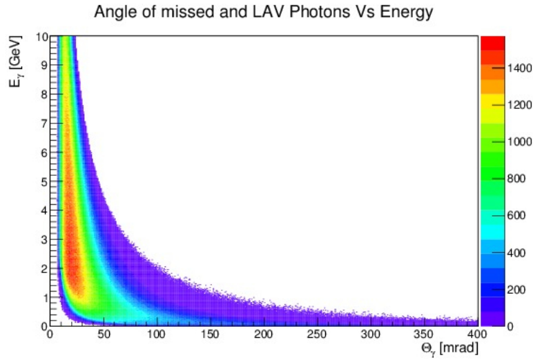
Figure 3. Energy vs decay angle ( E_\gamma vs \theta_\gamma ) of \pi^0 's daughter photons which pass outside the volume of the LKr. Note the extremely low energy of photons with decay angles greater than designed photon veto coverage (100 mrad).
