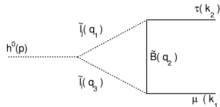
Figure 1. 1-loop SUSY slepton flavor mixing contribution to h^0 \rightarrow \mu \tau .
