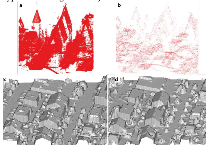
Figure 1. Building detection using different LiDAR data point clouds (Buffat R,2016)
