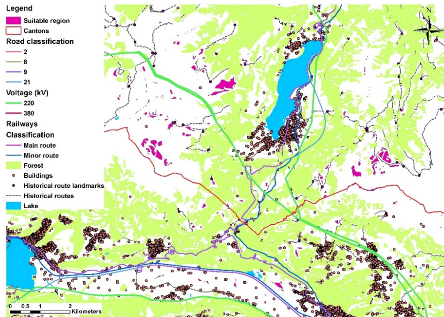
Figure 3. Identification of suitable areas far from constraints
