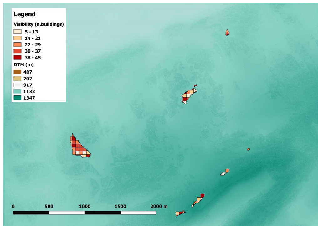
Figure 6. distribution of the number of visible buildings from each potential cell suitable for wind turbines.
