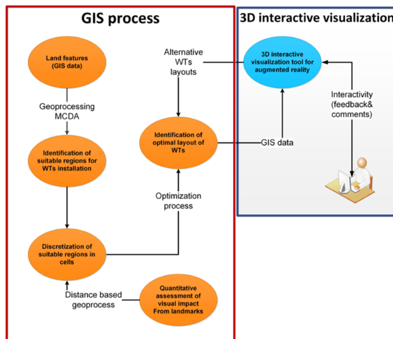
Figure 2. Geoprocessing of the developed platform for an augmented 3D interactive visualization of wind turbines
