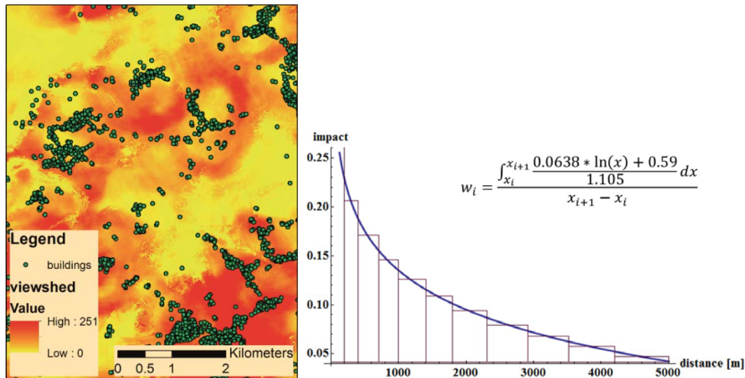
Figure 5. Spatial distribution of the visibility of transmission line towers from the buildings (left), approach used to estimate the visibility depending on the distance (right).
