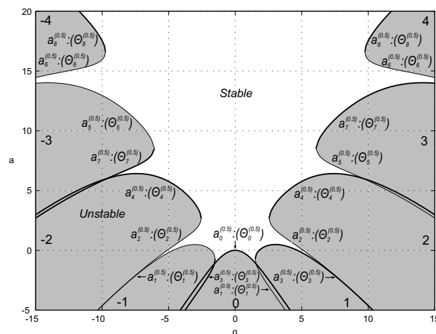
Figure 2. Eigenvalue curves of the fractional Mathieu equation ( c = 2 , \alpha = 0.5 ) calculated with Eq. (8) using r_{max} = 37 . Cross points of the curves represent degenerate eigenvalues of the fractional Mathieu equation. Unstable regions are numbered sequentially starting from the lowest curve.
