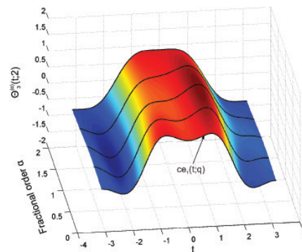
Figure 4. \Theta_3^{(\alpha)}(t;2) solution of the fractional Mathieu equation for \alpha \in [0, 2] . Solid curves correspond to \alpha = \{0, 0.5, 1, 1.5, 2\} .
