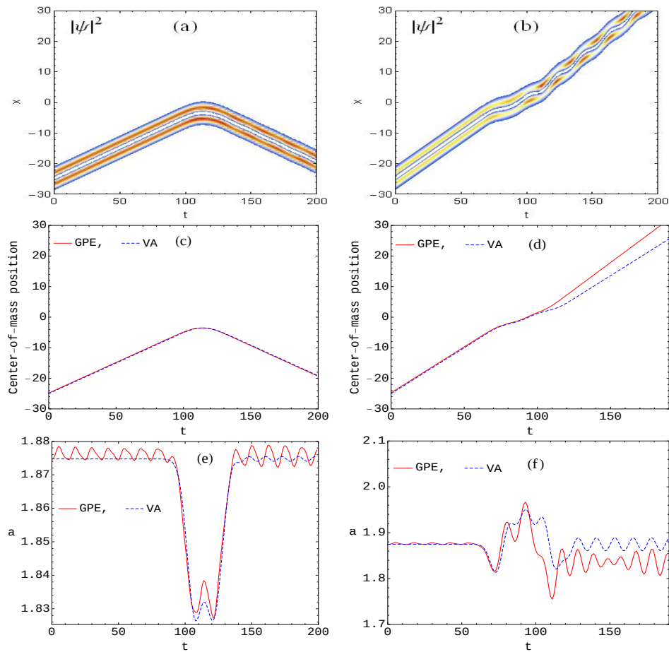
Figure 2. Scattering of a two-soliton molecule by weak potential barrier with V_0 = 0.1 at different velocities. Full reflection at low velocity v = 0.2 (a) and transmission at greater velocity v = 0.3 (b), according to GPE (1). Comparison GPE vs. VA for the center-of-mass position (c,d). At low velocity the two curves overlap (c), while at greater velocity there is a notable deviation after the scattering event (d). Agreement is only qualitative for the width (e,f). Initial parameter values A = 0.585 , a = 1.875 are predicted by VA for q = 0 , g = 20 , w = 5 , N = 2 , \xi_0 = -25 , d = 1 .
