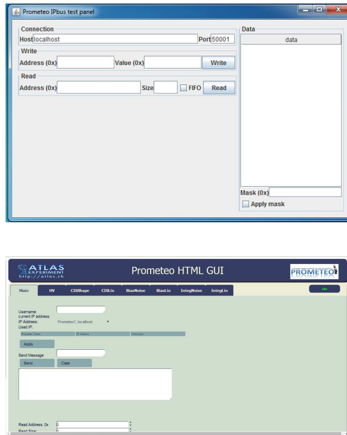
Figure 4. Top: Java GUI for Prometeo; Bottom: HTML GUI for Prometeo.
