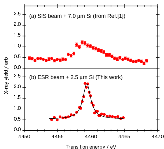
Figure 1. The RCE spectra of 2s-2p_{3/2} transition in the 190 MeV/u Li-like \text{U}^{89+} beam from (a) SIS and (b) ESR.
