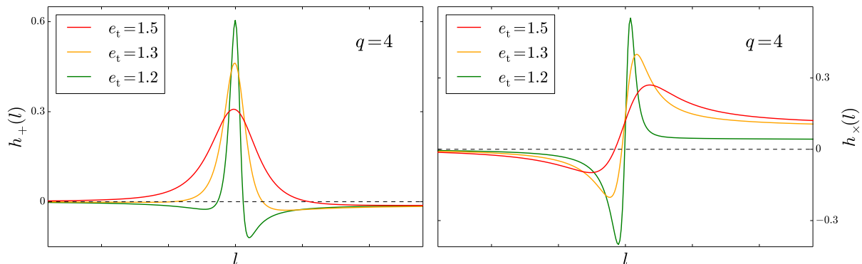
Figure 2. The gravitational wave signal of maximally spinning compact binaries on hyperbolic orbits, in units of Gm/c^2R , with mass ratio q = 4 , impact parameter b = 30 Gm/c^2 and for three different values of e_t . The orbital evolution is fully 1.5PN accurate and the influences of GW emission are taken into account. The linear memory effect causes the solid line waveform plots to depart from the dashed line after the hyperbolic passage.
