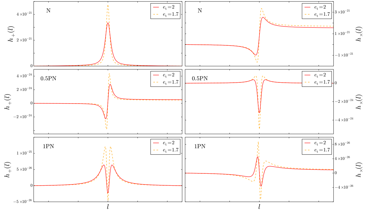
Figure 1. Polarization states at Newtonian, 0.5PN and 1PN order, as functions of the scaled time l for non-spinning compact binaries with periastron distance r_{min} = 1.9 \times 10^9 m and masses m_1 = 8M_\odot and m_2 = 13M_\odot , as in [4]. The non-vanishing amplitude of the \times polarization at late times, the so-called memory effect, is clearly visible at Newtonian order.
