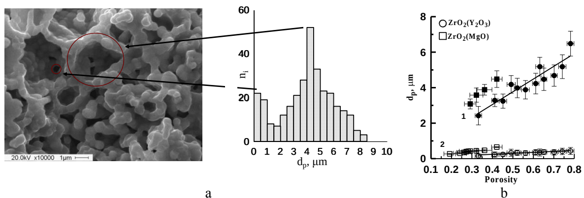
Figure 2. SEM-Picture of \text{ZrO}_2(\text{Y}_2\text{O}_3) ceramics structure, the characteristic pore size distribution of \text{ZrO}_2(\text{MgO}) ceramics with a porosity of \approx 40\% (a) and the dependence of the average pore size vs. porosity of \text{ZrO}_2 ceramics (b). 1) - the average size of large pores spherical-like shape; 2) - the average size of interparticle pores.
