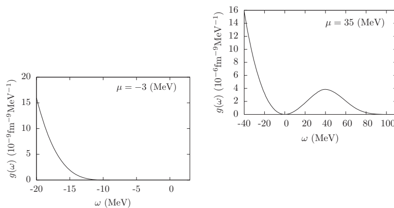
Figure 2. 3h level densities for negative and positive chemical potentials, respectively. Note that on the horizontal axis, the origine corresponds to \mu = 0 .
