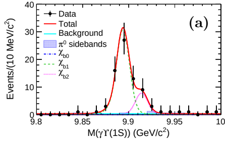
Figure 3. Projections of M(\gamma\Upsilon(1S)) (a) in the \omega signal region and (b) outside of \omega signal region, where the dash-dotted, dashed and dotted curves represent the \chi_{b0} , \chi_{b1} and \chi_{b2} signals, respectively.
