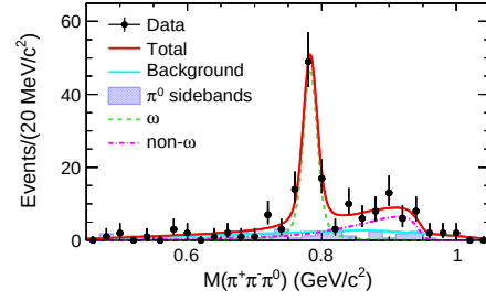
Figure 2. The M(\pi^+\pi^-\pi^0) invariant mass distribution, where the dashed and dash-dotted curves represent the \omega and (\pi^+\pi^-\pi^0)_{\text{non-}\omega} events; the hatched histogram is the normalized \pi^0 sideband events.
