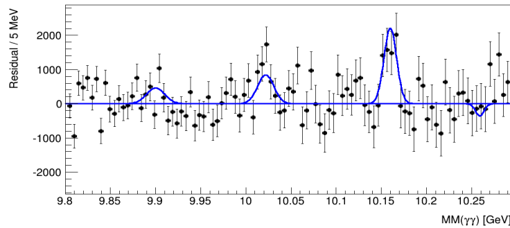
Figure 6. The \eta recoil mass distribution with the combinatorial background subtracted in the \Upsilon(5S) dataset. The blue curve represent the best fit.
