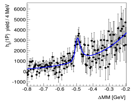
Figure 7. The \Delta MM distribution. The blue curve represents the best fit.
