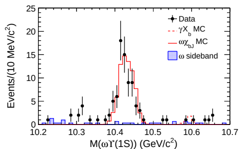
Figure 4. The \omega\Upsilon(1S) invariant mass distribution from selected \pi^0\pi^+\pi^-\gamma\Upsilon(1S) events.
