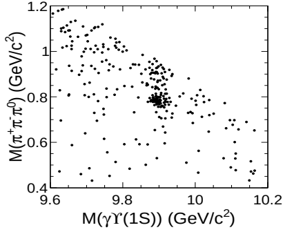
Figure 1. The scatter plot of M(\pi^+\pi^-\pi^0) versus M(\gamma\Upsilon(1S)) for selected e^+e^- \rightarrow \pi^+\pi^-\pi^0\gamma\Upsilon(1S) candidate events.
