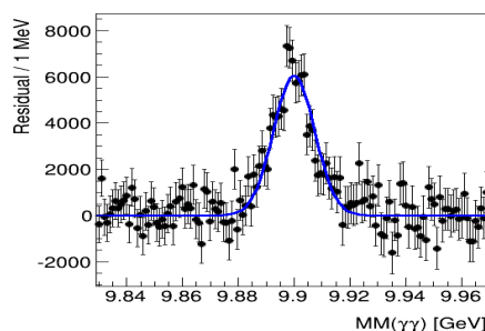
Figure 5. The \eta recoil mass distribution with the background subtracted in the \Upsilon(4S) dataset. The blue curve represents the best fit.
