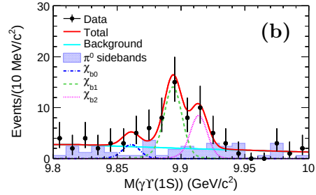
Figure 3. Projections of M(\gamma\Upsilon(1S)) (a) in the \omega signal region and (b) outside of \omega signal region, where the dash-dotted, dashed and dotted curves represent the \chi_{b0} , \chi_{b1} and \chi_{b2} signals, respectively.
