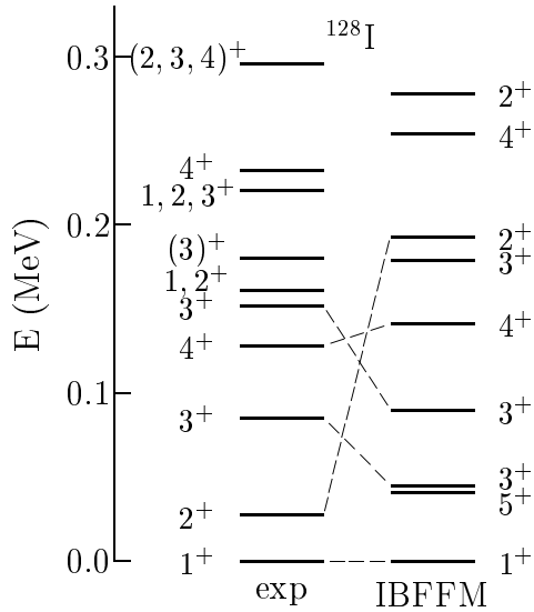
Figure 1. Energy levels in ^{128}\text{I} . The experimental data are from [18].
