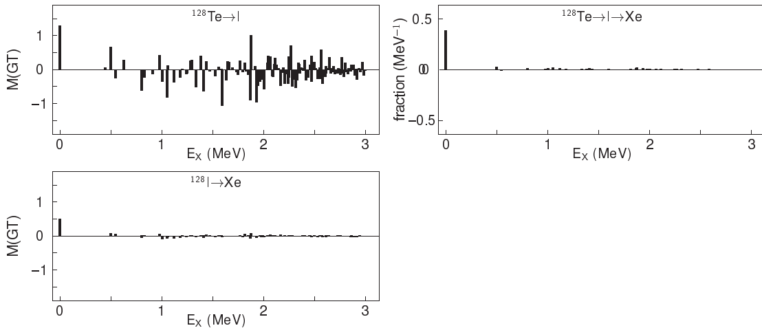
Figure 2. The values of \langle 1_N^+ || t^+ \sigma || 0_1^+ \rangle (top-left), \langle 0_1^+ || t^+ \sigma || 1_N^+ \rangle (bottom-left) and \langle 0_1^+ || t^+ \sigma || 1_N^+ \rangle \langle 1_N^+ || t^+ \sigma || 0_1^+ \rangle / (\frac{1}{2}(Q_{\beta\beta} + 2m_e c^2) + E_N - E_I) (top-right), for the double- \beta decay from the lowest 0^+ in ^{128}\text{Te} to the lowest 0^+ in ^{128}\text{Xe} through the intermediate 1^+ in ^{128}\text{I} , plotted as a function of the excitation energy.
