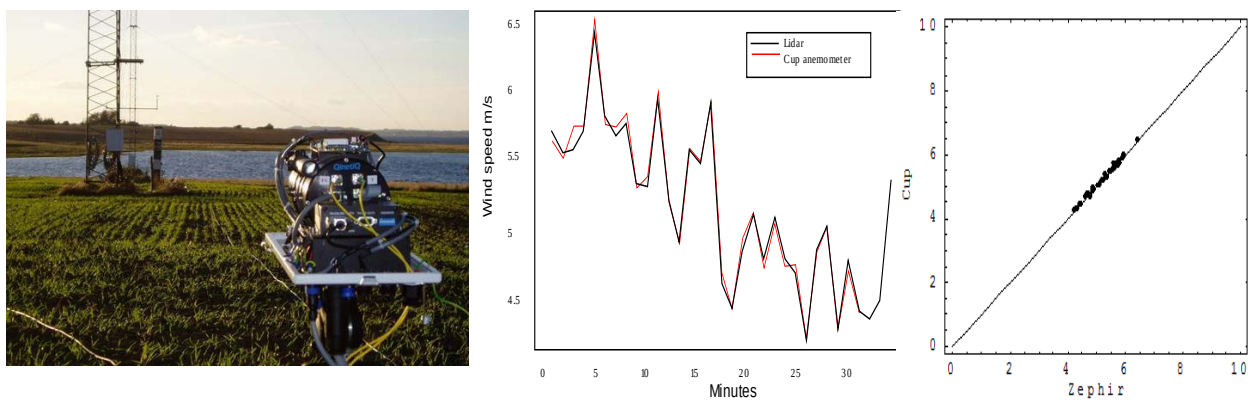
Figure 1. Left: “gray” QinetiQ all-fibre cw prototype lidar at test at Risø Campus October 14. 2003. Middle: measured time series of the lidar and the met mast cup at 60 m range. Right: scatter diagram between measured wind speeds from lidar vs cup anemometer.
