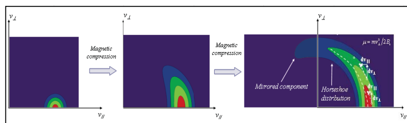
Figure 2 : Formation of the horseshoe in the electron velocity distribution
