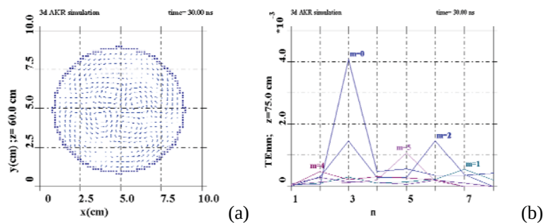
Figure 4: (a) 3D vector predictions of the transverse electric field patterns within the waveguide interaction region, the structure of a TE_{2,3} mode is clearly seen at 11.7GHz. (b) illustrates the results of the transverse spatial Fourier analysis output predicted by KARAT 3D for the 11.7GHz resonance.
