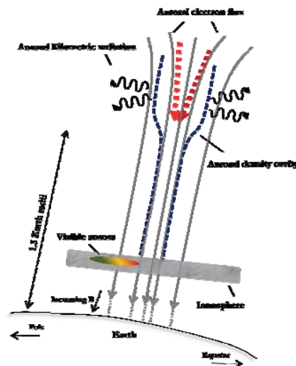
Figure 1: Representation of the AKR source region and terrestrial auroral process.
