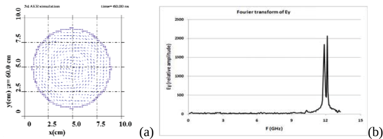
Figure 5: (a) Illustrates excitation of TE_{0,3} mode. (b) shows a peak at \sim 11.7 GHz along with another at \sim 12.2 GHz, this is illustrative of multiple modes being excited and mode competition.
