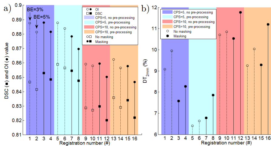
Figure 1. Variation of a) DSC (squares) and OI (circles) and b) DT_{2mm} for different combinations of parameters: BE=3% (#1,3,5,7,9,11,13,15) and BE=5% (#2,4,6,8,10,12,14,16); CPS=5 (#1-8) and CP=10 (#9-16); mask (#3,4,7,8,11,12,15,16) and no mask (#1,2,5,6,9,10,13,14); pre-processing (#5-8,13-16) and no-preprocessing (#1-4,9-12). Smaller control point spacing translated in larger values of DSC and OI. Pre-processing the CBCT improved DSC and DT_{2mm} values.
