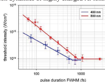
Figure 1. Evolution of the intensity threshold as a function of the pulse duration for two laser wavelengths and a cluster size close to 10^5 at/cl.
