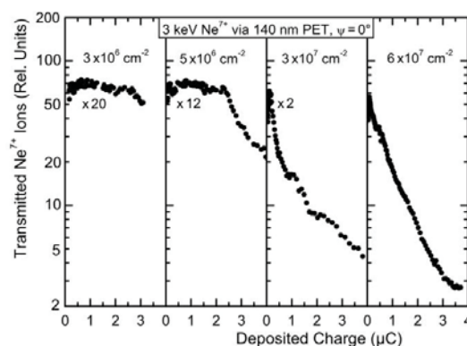
Figure 1. Number of transmitted \text{Ne}^{7+} ions as a function of the deposited charge for a tilt angle of \psi = 0^\circ . The capillary density is indicated in each panel. The capillary diameter amounts to 140 nm.
