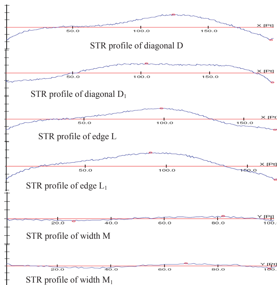
Figure 5. Result of STR form for D&D 1 , L&L 1 ; M&M 1 lines for third specimen using new method
