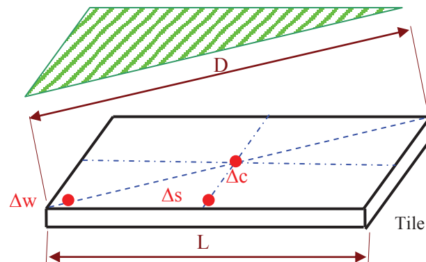
Figure1. The position schematic of the centre points \Delta s , \Delta c ; \Delta w and 3 points plane.
