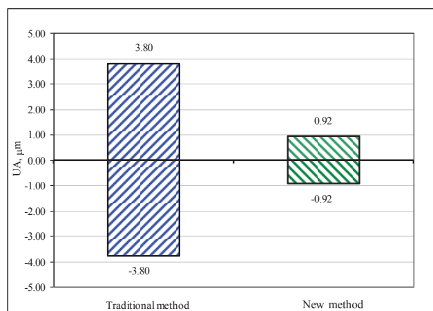
Figure 8. Expanded uncertainty for traditional and new obtained methods
