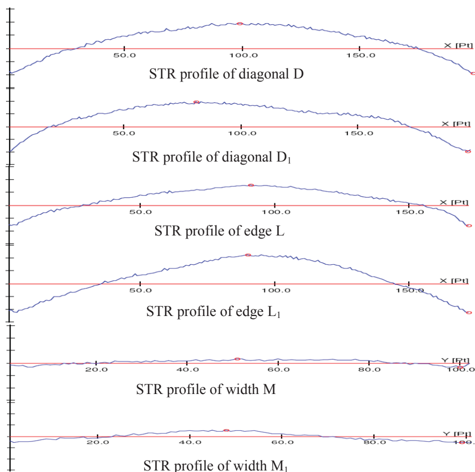
Figure 4. Result of STR form for D&D 1 , L&L 1 ; M&M 1 lines of second specimen in the new method
