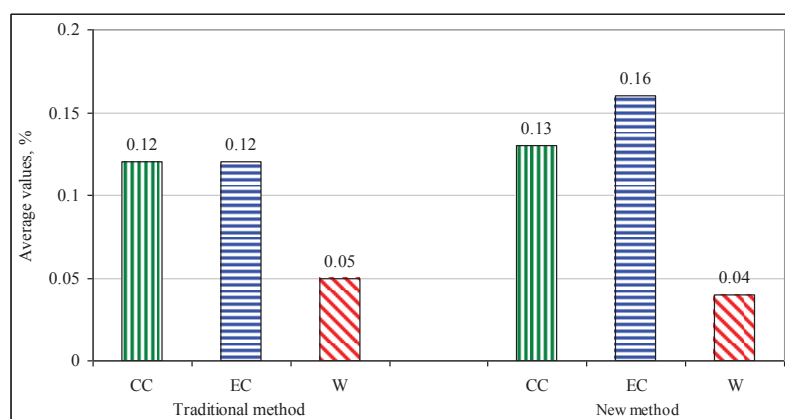
Figure 7. Results of important specific parameters using traditional method and new method
