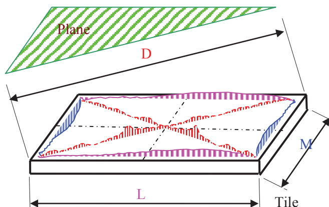
Figure 2. The positions of STR measurement for D, D 1 , L, L 1 , M; M 1 and 3 points plane
