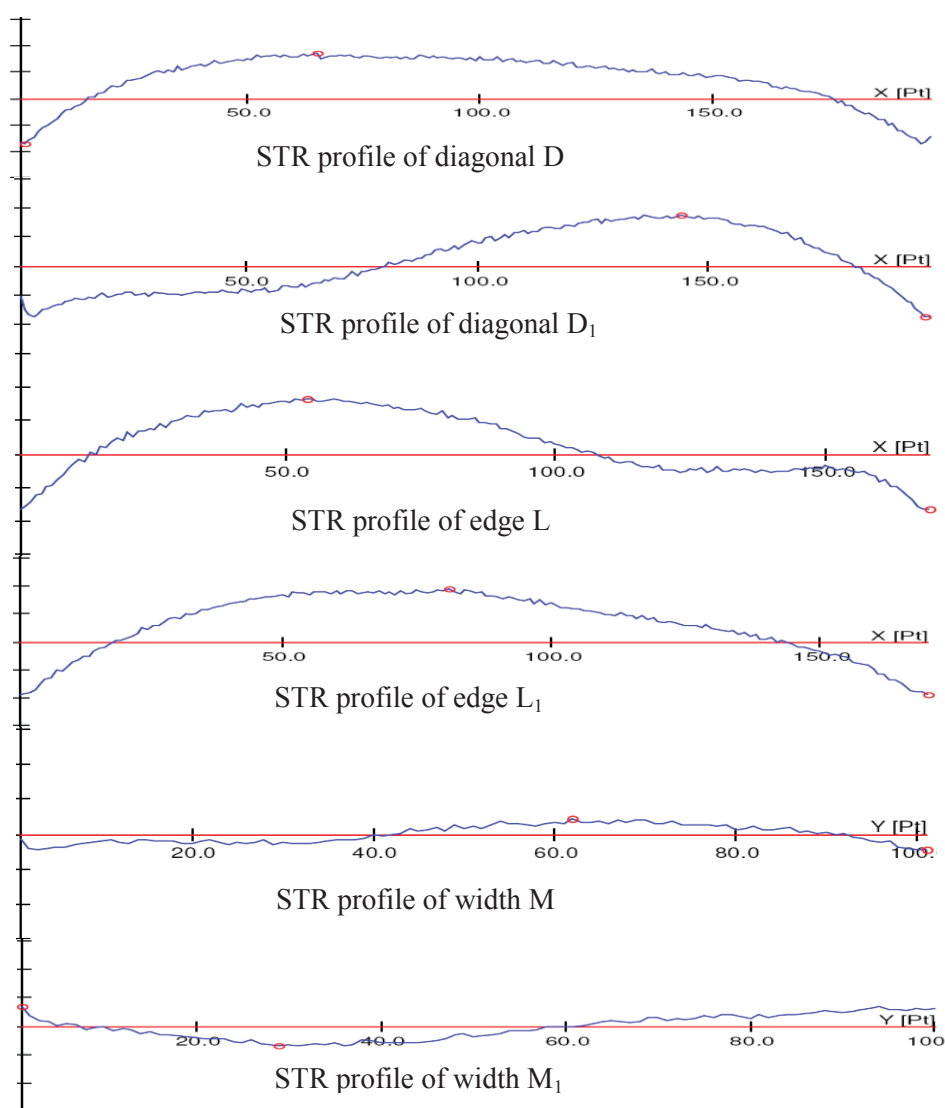
Figure 3. Sample result of STR for D&D 1 , L&L 1 ; M&M 1 lines for tile first specimen using new method
