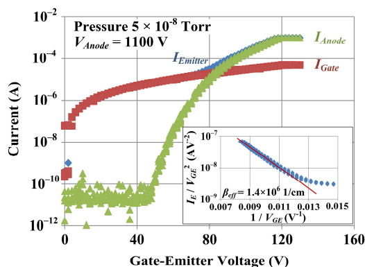
Figure 3. Transfer characteristics of FEN; inset shows linear FN behavior with field factor > 10^6 .
