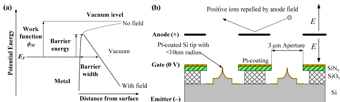
Figure 1. (a) Potential energy diagram of electrons at the vicinity of a metal surface w/o normal electrostatic incident field. (b) Cross-section schematic of field emission neutralizer; the electric field direction is shown with a metal mesh used as anode.
