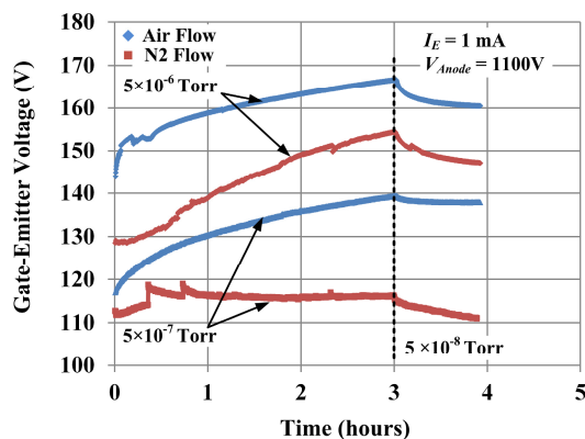
Figure 5. Field emission at 5 \times 10^{-6} and 5 \times 10^{-7} Torr in both N_2 and air atmospheres. Device degradation was reversible after operation in N_2 at 5 \times 10^{-7} Torr.
