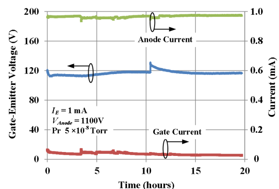
Figure 4. Long-term FEN performance: gate-emitter voltage, anode current, and gate current over time for a device emitting 1 mA.
