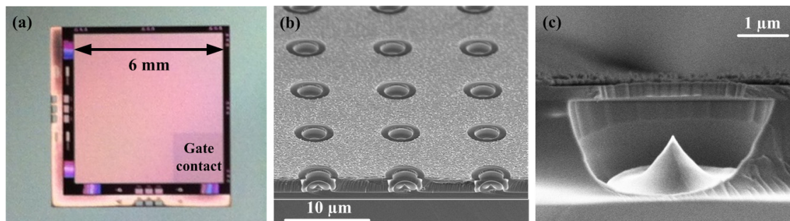
Figure 2. (a) Optical image of a field emitter neutralizer; (b) angle-view and (c) cross-section SEM images of self-aligned gated tips.
