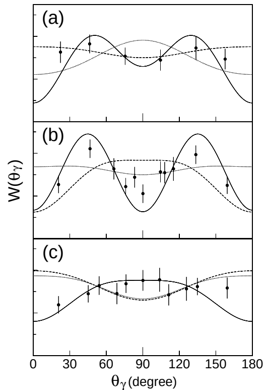
Figure 4. Angular correlations for three quantization z axes (see text for the axes). Solid lines are those of the molecular ground state, dashed lines for the first excited state and dotted lines for the second excited state.
