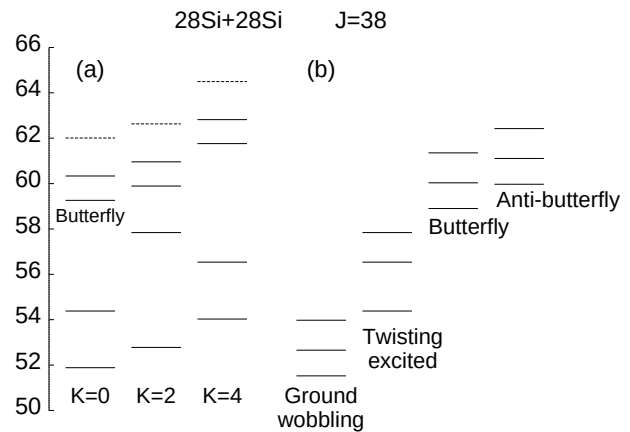
Figure 3. Energy spectra of the ^{28}\text{Si} + ^{28}\text{Si} system for J = 38 . (a) Molecular normal modes without K -mixing. (b) After K -mixing, with indications of the modes under the levels.
