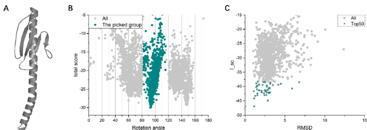
Figure 1. (A) the full-length structure of S. oneidensis pili; (B) the landscapes of energy score versus rotation angle of subunits at the end of the first step; (C) the interfacial energy score versus RMSD of the refined models after the second step.
