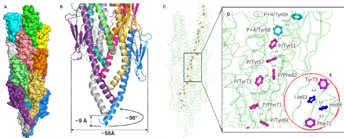
Figure 2. The model with the lowest interfacial energy. (A) the filament model containing 15 subunits; (B) the symmetry parameters, i.e. the rotation angle, axial rise and diameter of the model; (C) a potential pathway formed by aromatic rings; (D) details of the neighbouring aromatic rings; (E) suggested mutations that would fill the gap of the pathway, with mutated residues in blue.
