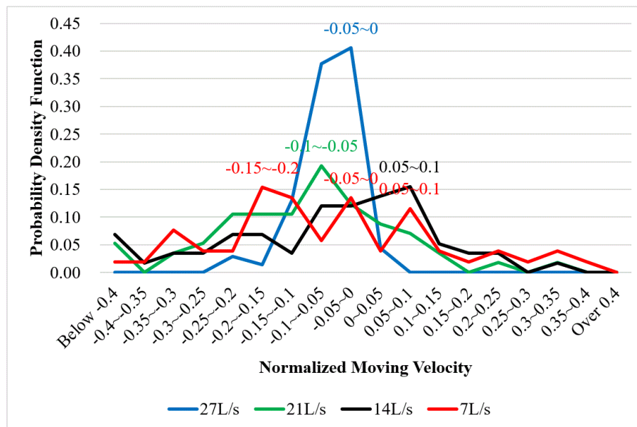
Figure 7. Normalized moving velocity distribution of backflow vortices on casing
