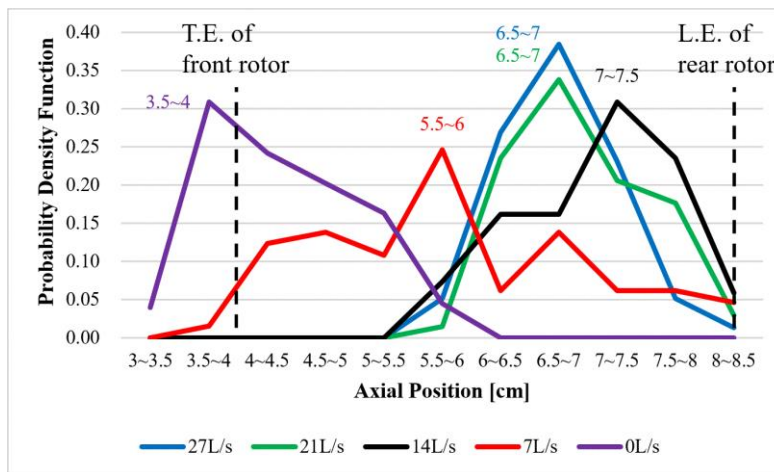
Figure 5. Axial position of backflow vortex cores on casing
