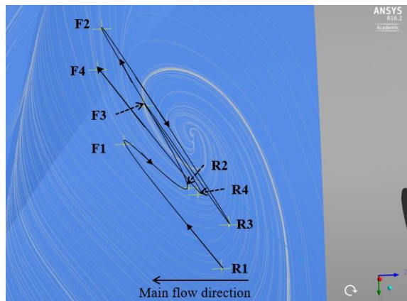
Figure 8. Trajectory of one vortex at flow rate 0L/s
