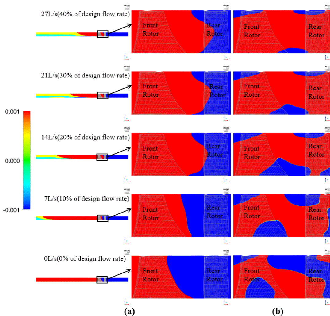
Figure 4. Contours of averaged normalized circumferential (a) and axial (b) velocities
