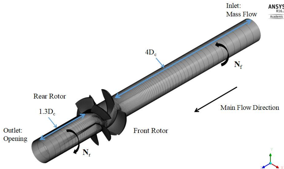
Figure 1. Numerical model
