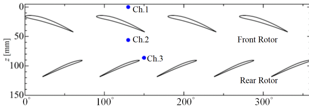
Figure 2. Pressure taps position
