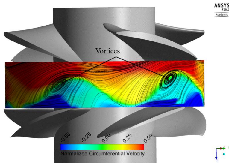
Figure 3. Vortex structures and normalized circumferential velocity distribution on 0.975 span at 30% of design flow rate
