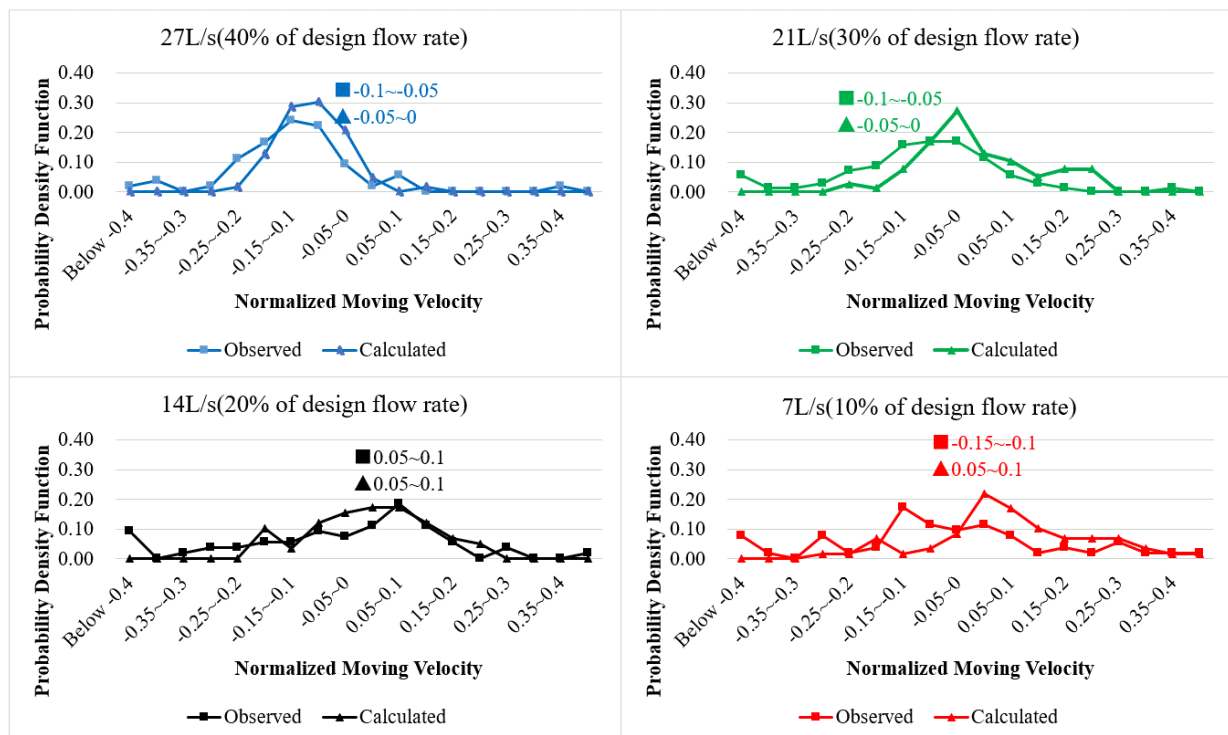
Figure 6. Comparison of the velocity observed and calculated with circumferential velocities of main flow and backflow
