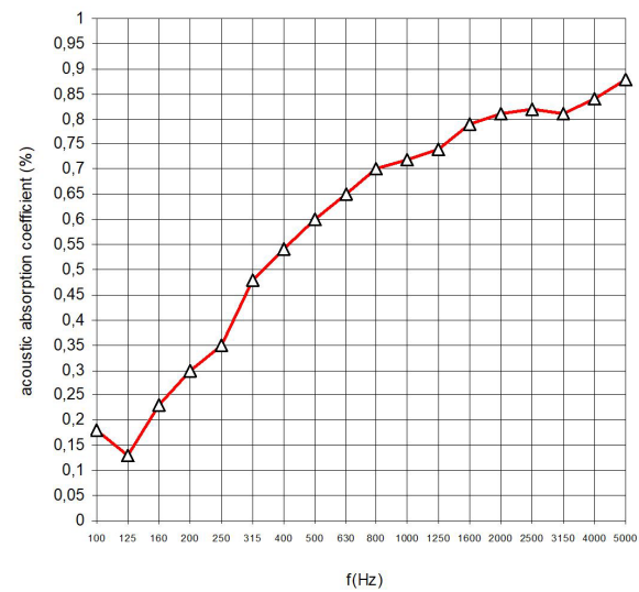
Figure 8. Acoustic absorption coefficients \alpha_s (%), obtained in conformity with EN ISO 354, for sample P7
