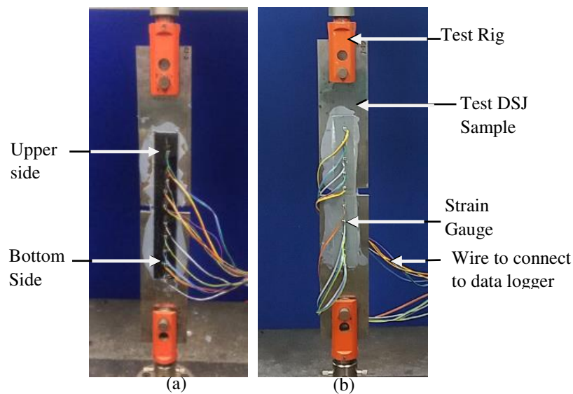
Figure 2: Sample double strap joints (DSJ) under tensile load for (a) CFRP-Steel and (b) GFRP-Steel
