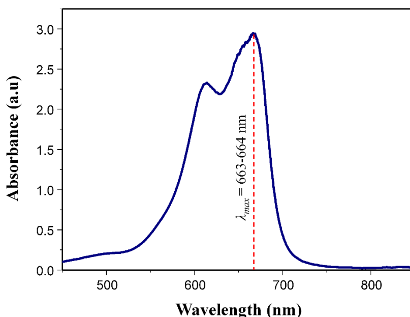
Figure 2. UV-Visible absorbance spectrum of Methylene blue.
