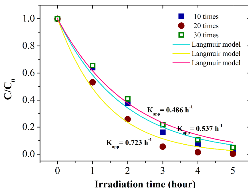
Figure 4. The effect of spray number in catalyst performance toward kinetic rate of photocatalyst activity, blue curve represents the sprayed catalyst of 10 times, yellow curve represents the sprayed catalyst of 20 times, and pink curve represents the sprayed catalyst of 30 times.
