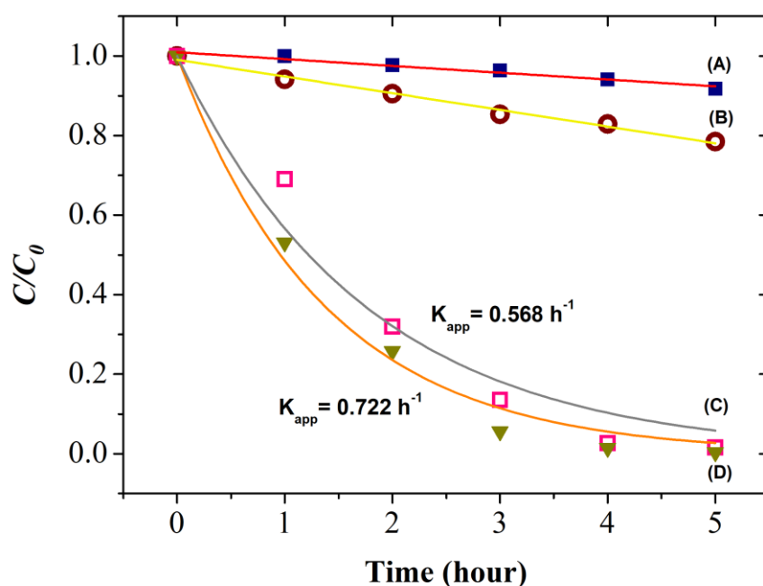
Figure 3. The degradation level of MB after treatment by (A) \text{TiO}_2 without irradiation; (B) irradiation without catalyst used; (C) \text{TiO}_2 -coated plastic using spraying method without heat treatment; and (D) \text{TiO}_2 -coated plastic using spraying method combined with heat treatment.
