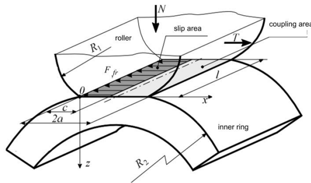
Figure 2. Calculation diagram of the roller-ring contact model.
