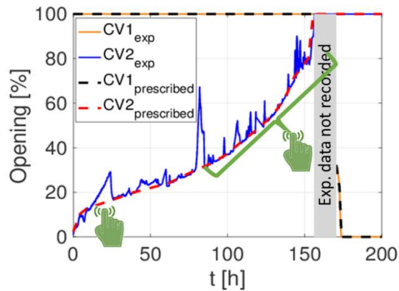
Figure 3. Evolution of the opening of the control valves CV1 and CV2, as resulting from a combination of automatic and manual (👉) controls.
