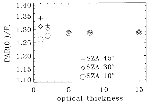
Figure 5. Ratio between the plane flux just above the sea surface and PAR below the sea surface as a function of the optical thickness.
