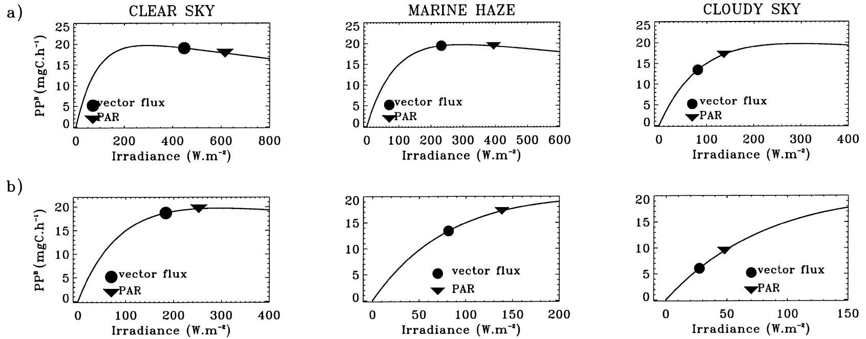
Figure 6. The integrated vector fluxes and PAR are shown on P-I curve for different atmospheric conditions (clear sky, marine haze and cloudy sky) and depth a) 5 m, b) 10 m for a zenith solar angle equal to 30^\circ .
