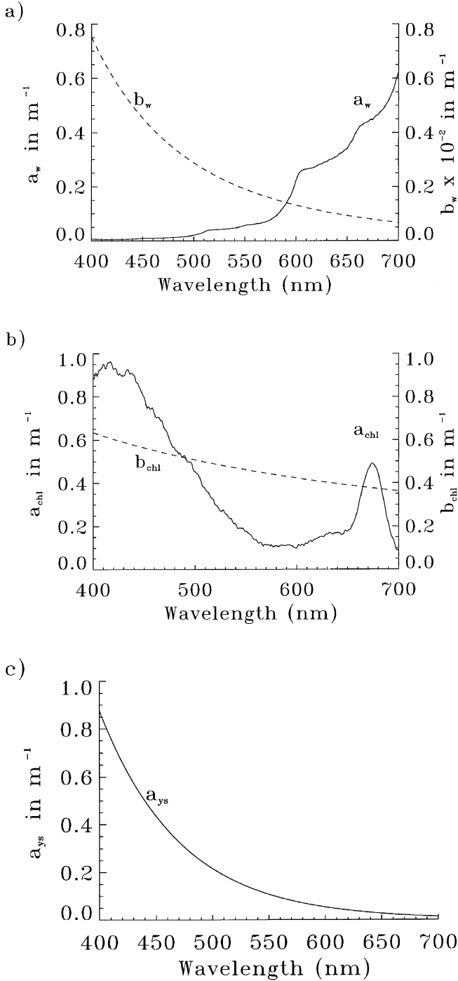
Figure 2. Absorption (solid line) and scattering (dashed line) coefficient for a) pure sea water, b) suspended chlorophyllous matter and c) yellow substances.
