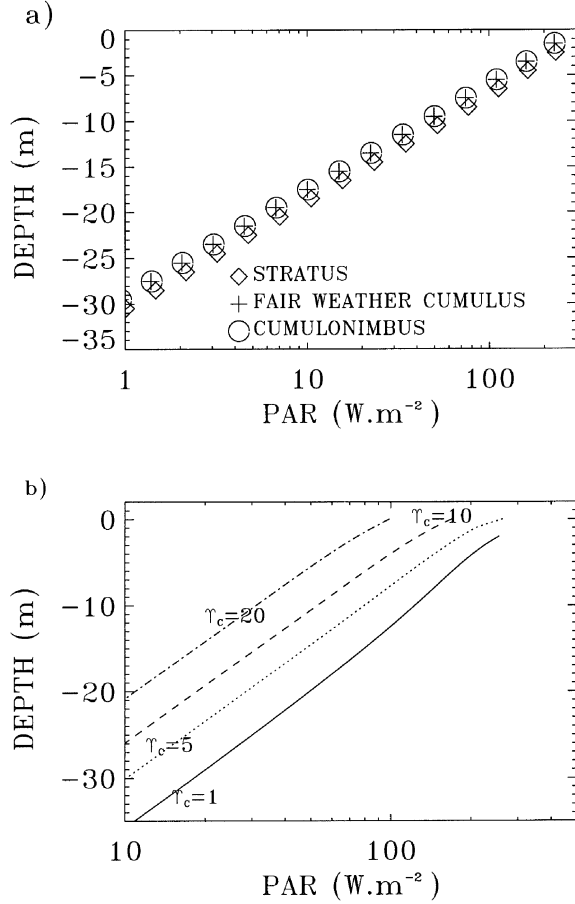
Figure 4. a) Distribution of PAR ( \text{W.m}^{-2} ) on the water column for 3 types of clouds: stratus (diamond), fair weather cumulus (cross) and cumulonimbus (circle); b) distribution of PAR on the water column in a cloudy atmosphere for various optical thicknesses.
