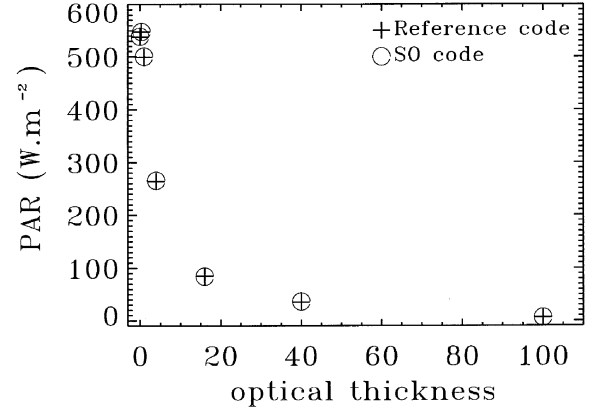
Figure 3. Comparison between a reference code (GAME) and the SO code for a cloudy atmosphere.
