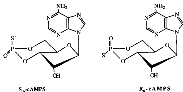
Fig. 1. Chemical structures of ( R_p )-cAMPS and ( S_p )-cAMPS.
