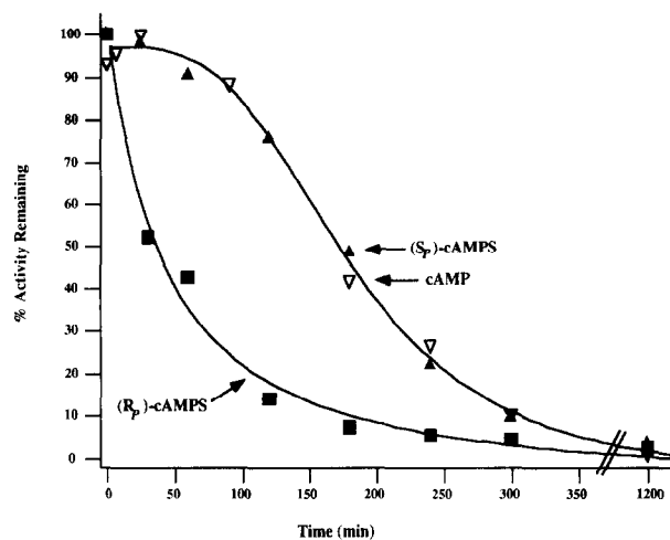
Fig. 4. Time course of holoenzyme formation in the presence of MgATP by equilibrium dialysis at room temperature. The remaining phosphotransferase activity of unbound catalytic subunit was measured [26] and plotted against the time of dialysis. Prior to the dialysis regulatory subunit was stripped off cAMP as described in section 2, reloaded by either an excess of cAMP ( \nabla ), ( R p )-cAMPS ( \blacksquare ) or ( S p )-cAMPS ( \blacktriangle ) and mixed with C-subunit in a 1:1.1 molar ratio.
