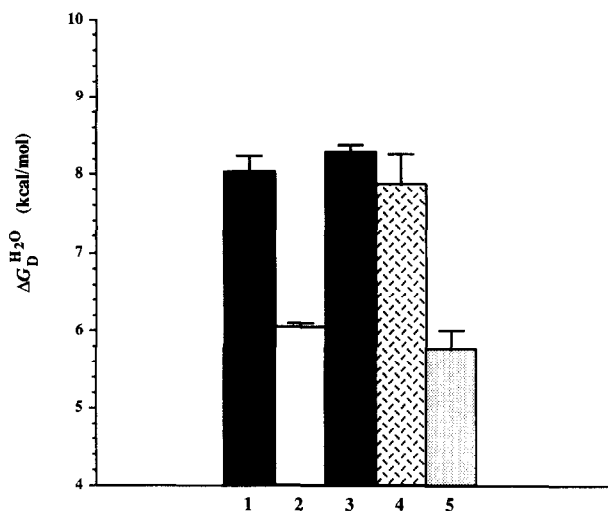
Fig. 3. Free energy changes ( \Delta G_D^{\text{H}_2\text{O}} ) were calculated by linear regression of the unfolding transition data (inset of Fig. 2) according to equation (3). Panel 1: native R-subunit; panel 2: urea stripped, cAMP-free R-subunit; panel 3: urea stripped R-subunit + excess cAMP; panel 4: urea stripped R-subunit + excess ( S p )-cAMPS; panel 5: urea stripped R-subunit + excess ( R p )-cAMPS. In the experiments described in panel 3–5, the cyclic nucleotides were added prior to denaturation.
