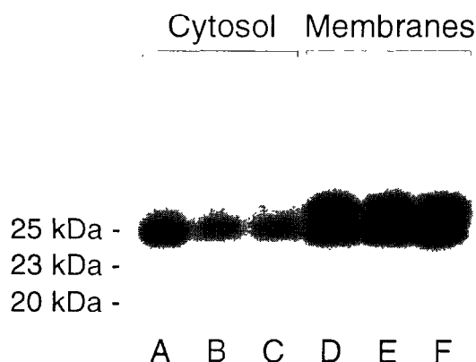
Fig. 5. Subcellular distribution of small G-proteins at various times after permeabilization of HIT cells. The cells were washed twice and either directly homogenized (A,D) or treated with 1 U/ml SL-O for 8 min (B,C,E,F). Before homogenization, the permeabilized cells were incubated for 24 min at 100 nM free \text{Ca}^{2+} , with (C,F) or without (B,E) 100 \mu M GTP \gamma S included during the last 8 min incubation. The cytosolic and crude membrane fractions were then prepared as previously described [9,22]. The SMGs present in the two fractions were revealed using the GTP-overlay technique [9,22]. Two bands detected on the films were quantified by densitometric scanning. The values obtained for the 23 kDa and 25 kDa bands were respectively (arbitrary units, mean of two determinations): lane A, 1,680 and 4,829; lane B, 1,125 and 3,154; lane C, 1,261 and 3,277; lane D, 2,713 and 4,964; lane E, 2,300 and 4,981; and lane F, 2,522 and 5,284.
