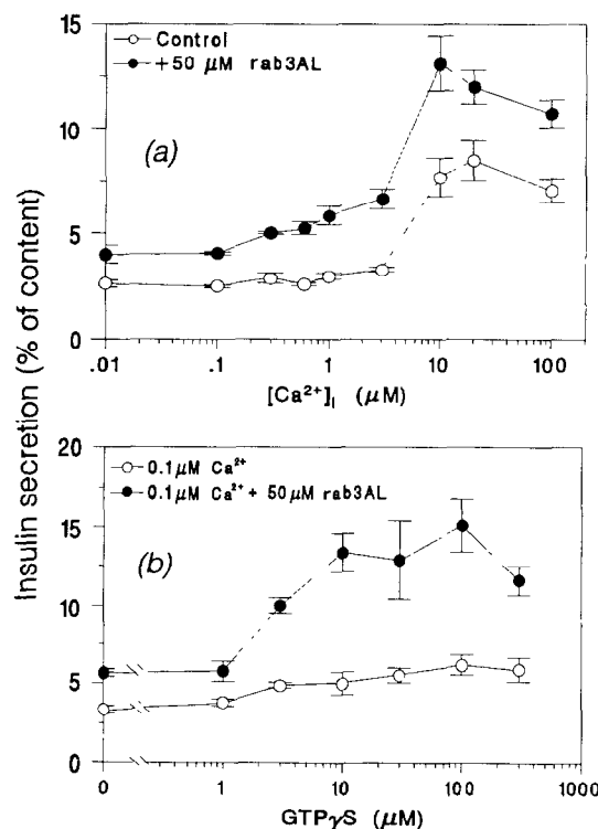
Fig. 2. Effect of rab3AL peptide on Ca 2+ - and GTPγS-induced insulin secretion from SL-O permeabilized HIT cells. Values are mean ± S.E.M. of four experiments. For experimental detail, see legend to Fig. 1.
