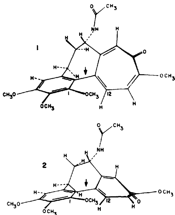
Fig.3. Multiple conformations of colchicine. Four different conformations are possible. Conformation 2 shown above is related to conformation 1 by a boat-boat interconversion of the troponoid C-ring. The dihedral angle between the plane defined by C_{7a} , C_{11} , C_{12} and C_{12a} of the C-ring and the planar A-ring is about 53^\circ . This dihedral angle is reduced to 19^\circ in conformation 2. Two other conformations of colchicine are possible which are related to the shown C-ring boat-boat conformers by atropisomerism (about the biaryl bond \downarrow ). Although such atropisomerism leads to change the chirality of the biaryl moieties, there is no change in the dihedral angles. (Reproduced with permission from the American Chemical Society.)
