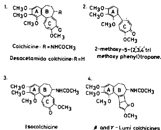
Fig.1. Structure of colchicine and its analogues.
