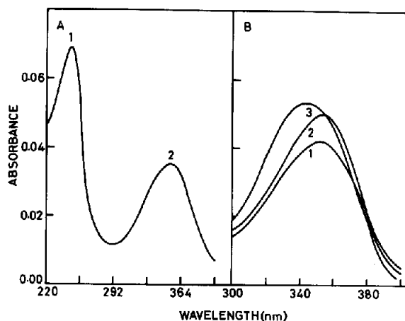
Fig.2. (A) Ultraviolet absorption spectra of colchicine ( 2.27 \times 10^{-6} M) in water. Absorption maxima: \lambda_{\text{max}1} = 247 nm; \lambda_{\text{max}2} = 353 nm. (B) Absorption spectra of colchicine ( 2.7 \times 10^{-6} M), desacetamidocolchicine ( 2.8 \times 10^{-6} M) and AC compound ( 3 \times 10^{-6} M) in assembly buffer. (1) Colchicine, \lambda_{\text{max}} = 353 nm; (2) desacetamidocolchicine, \lambda_{\text{max}} = 353 nm; (3) AC compound, \lambda_{\text{max}} = 341 nm.
