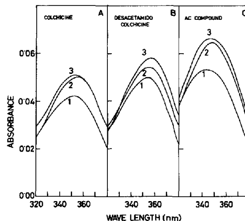
Fig.4. Absorption spectra of colchicine, desacetamidocolchicine and AC compound in assembly buffer (1), in 100% glycerol (2) and in the presence of tubulin (3). In (3), the drugs are incubated with a 5-fold excess of tubulin ( 15 \mu\text{M} ) in assembly buffer without GTP at 37^\circ\text{C} for 30 min. (A) Colchicine ( 2.7 \times 10^{-6} \text{ M} ). \lambda_{\text{max}} : (1) 353 nm, (2) 358 nm, (3) 354 nm. (B) Desacetamidocolchicine ( 2.8 \times 10^{-6} \text{ M} ). \lambda_{\text{max}} : (1) 353 nm, (2) 355 nm, (3) 356 nm. (C) AC compound ( 3 \times 10^{-6} \text{ M} ). \lambda_{\text{max}} : (1) 341 nm, (2) 348 nm, (3) 346 nm.
