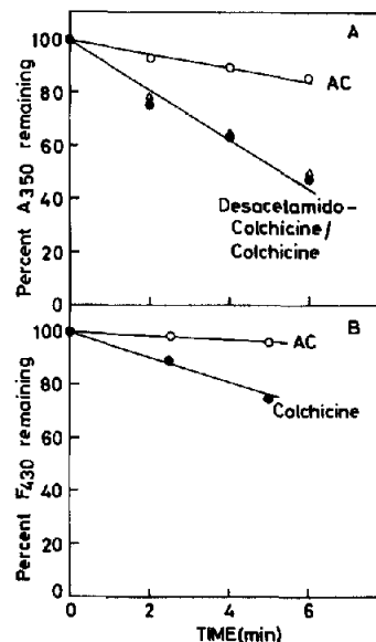
Fig.6. (A) Time kinetics of ultraviolet-induced rearrangement of colchicine, desacetamidocolchicine and AC compound in 95% ethanol. The ultraviolet irradiation experiment was done as described in section 2. (B) Time course of release of drug from drug-tubulin complex (measured by decrease in fluorescence at 430 nm) during irradiation with ultraviolet light. 2.5 \mu M tubulin was incubated with 5 \mu M drug at 37°C for 30 min. The resultant drug-tubulin complex was irradiated for the indicated times and the fluorescence at 430 nm was measured.
