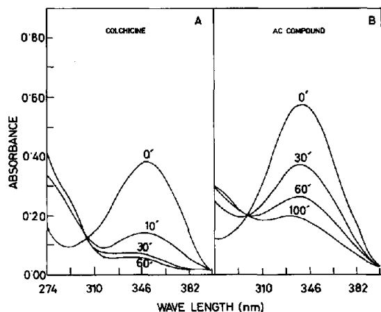
Fig.5. Absorption spectra of colchicine and AC compound at different time intervals during irradiation with ultraviolet light. The irradiation experiment was carried out as described in section 2. (A) Colchicine, isosbestic point, 303 nm. (B) AC compound, isosbestic point, 292 nm.
