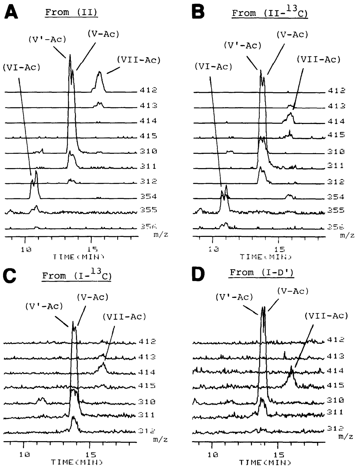
Fig.1. Mass chromatogram of molecular ion peaks of degradation products from (II), (II- 13 C), (I- 13 C) and (I-D') by the lignin peroxidase/H 2 O 2 system. (A) Degradation products from unlabeled 4-ethoxy-3-methoxyphenylglycerol-β-
