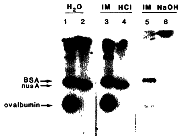
Fig.4. Adduct stability in acid and base. BSA and ovalbumin (lanes 1, 3, and 5) and nusA protein (lanes 2, 4, and 6) were labeled with [ \alpha - ^{32} P]CTP as described in section 2. Gel slices were soaked with agitation for 15 h at 25°C as indicated prior to autoradiography.
