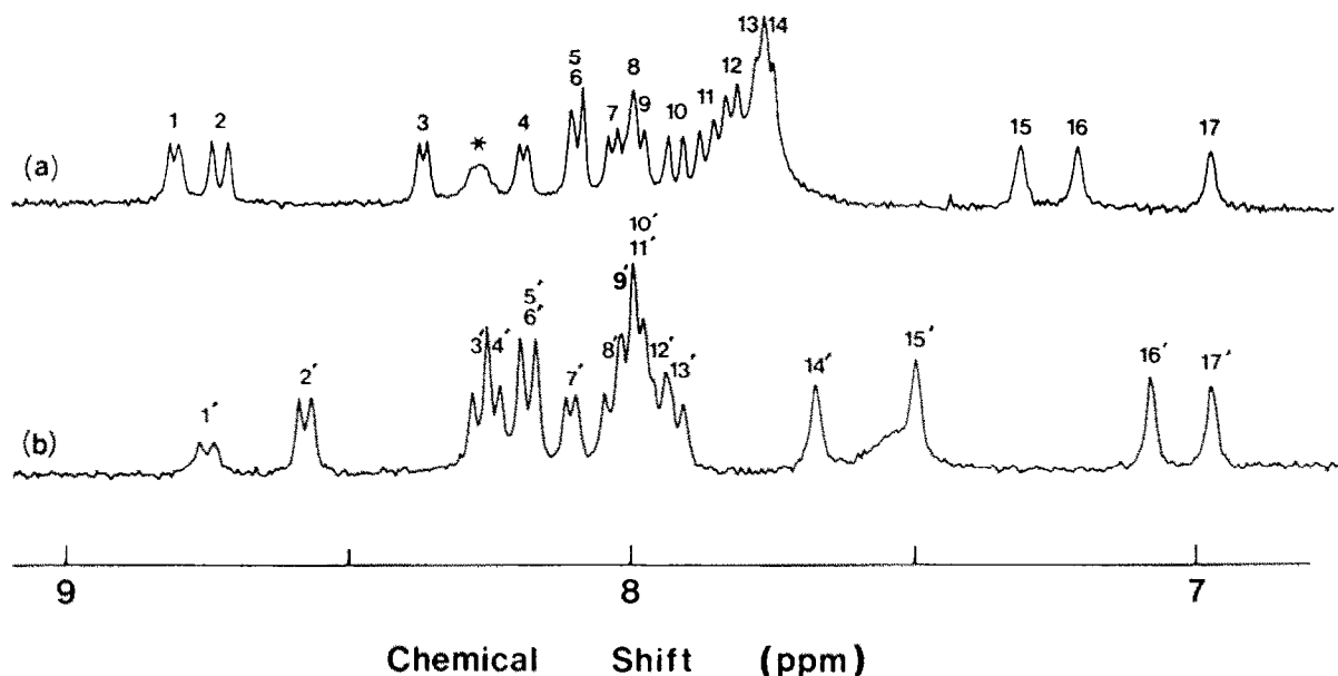
Fig.3. The 270-MHz ^1\text{H} -NMR spectra (in the NH proton region) of mastoparan (2 mM, 23^\circ\text{C} ) in \text{C}^2\text{H}_3\text{OH} solution (a) and in \text{H}_2\text{O} solution at pH 4 (b). The chemical shifts (ppm) are measured downfield from the internal standard of 2,2-dimethyl-2-silapentane-5-sulfonate. The strong solvent resonances are pre-saturated by irradiation for 0.5 s prior to the observation pulse. The peak * in (a) is due to the \alpha\text{-NH}_3^+ group of mastoparan which has been prepared by lyophilization of the aqueous solution at pH 3.5.
