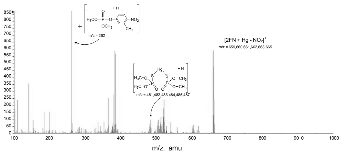
Figure 3. Positive ion ESI-MS spectrum of 50% aqueous methanol solution containing 5.0 \times 10^{-5} M FN and 2.5 \times 10^{-4} M \text{Hg}^{2+} ion.
