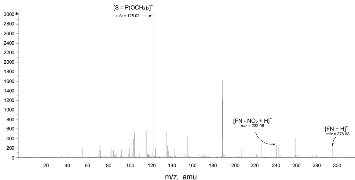
Figure 2. MS/MS (CID) spectrum of [\text{FN}+\text{H}]^+ ( m/z = 278.08 ), which fragments into various ions, collision energy and collision gas pressure were 65 eV and 3.0 \times 10^{-3} Pa, respectively.
