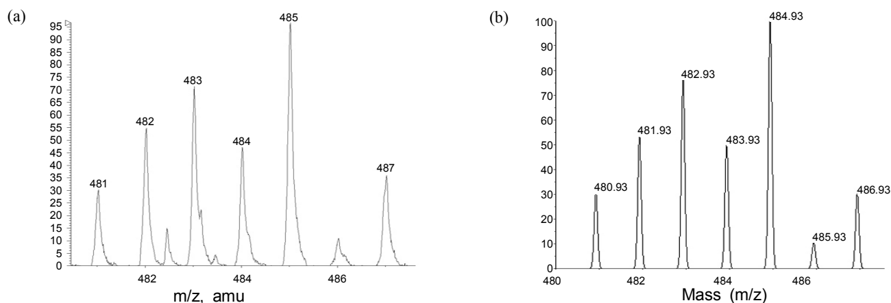
Figure 4. A representative figure showing the agreement between the experimental (a) and the theoretical (b) peaks corresponding to [2\{\text{S-P}(=\text{O})(\text{OCH}_3)_2\} + \text{Hg} + \text{H}]^+ ion from ESI-MS of FN and \text{Hg}^{2+} .
