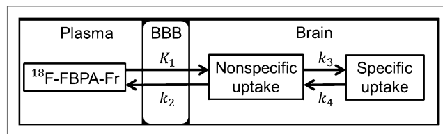
FIGURE 1. Pharmacokinetics of ^{18}\text{F} -FBPA-Fr analyzed by 3-compartment model for K_1 (mL/g/min), k_2 ( \text{min}^{-1} ), k_3 ( \text{min}^{-1} ), and k_4 ( \text{min}^{-1} ). K_1 and k_2 represent forward transport and reverse transport of ^{18}\text{F} -FBPA-Fr across BBB, respectively. k_3 and k_4 are anabolic and reverse-process rate constants, respectively.
