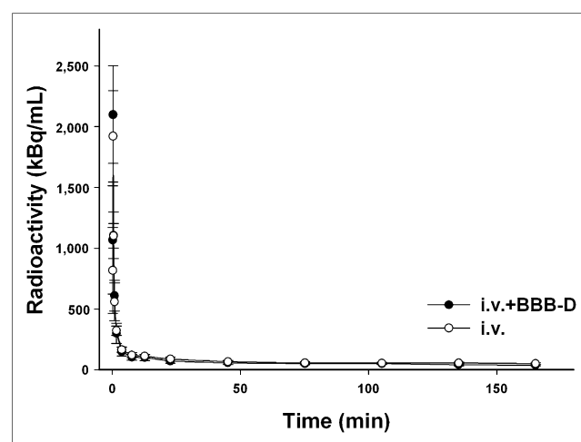
FIGURE 4. Time-activity curves for ^{18}\text{F} -FBPA-Fr in plasma of F98 glioma-bearing rats after intravenous (i.v.) injection of ^{18}\text{F} -FBPA-Fr both with and without BBB-D. Each point represents mean \pm SEM for 5 rats.
