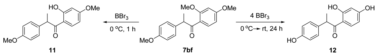
Scheme 3. Demethylation of 7bf using boron tribromide.
