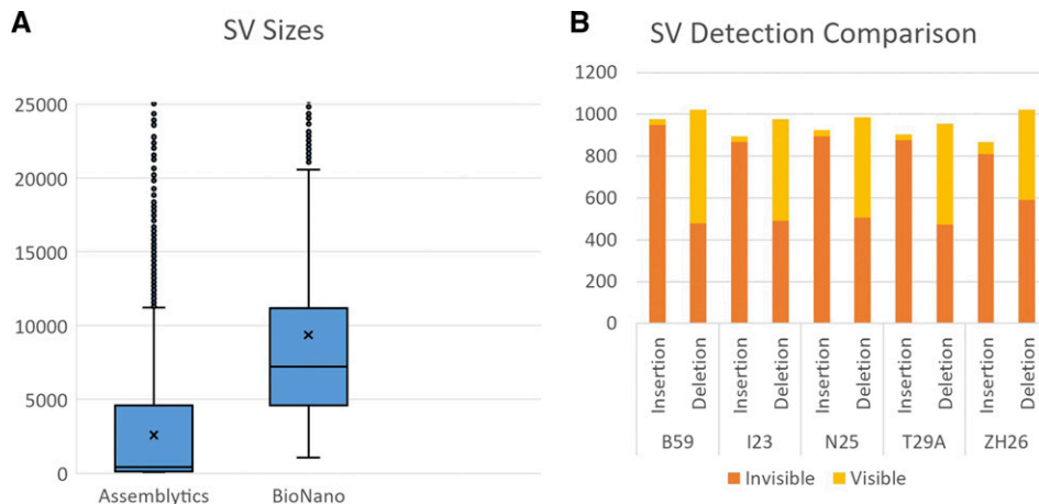
Figure 3 A) Size distribution of structural variants called by both long-read sequencing and Optical Map methods. The Y-axis is defined to show majority of variance and does not display some larger SVs detected. B) Sequence SVs detected by long-read sequencing, but not by short read resequencing are classified as "invisible".
