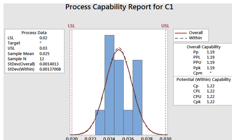
Fig. 4 Process capability graph of optimal parameters
