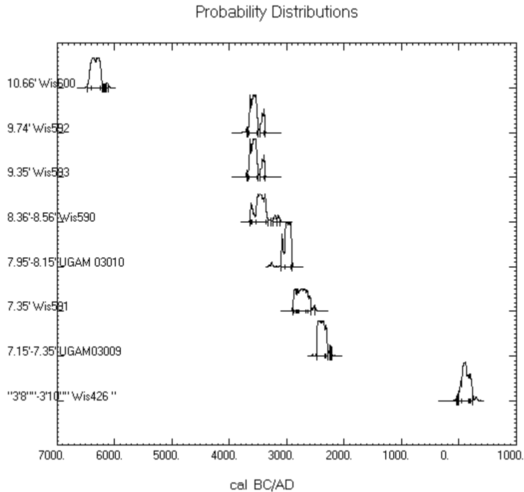
Image 1: Probability Distributions
