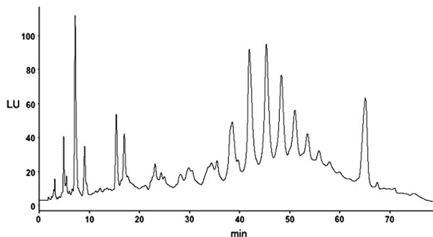
Fig. 2. Normal-phase HPLC chromatogram (with fluorescence detection) of a DP7+ cocoa PC fraction.
