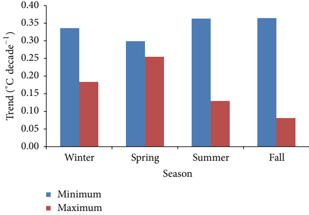
FIGURE 2: Seasonal trends (°C decade -1 ) for maximum and minimum temperatures.
