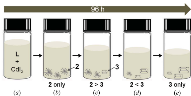
Figure 3 Cartoon presentation of time-dependent crystal growth, dissolution and recrystallization in the mother solution: 2 forms needles and 3 forms bricks.
