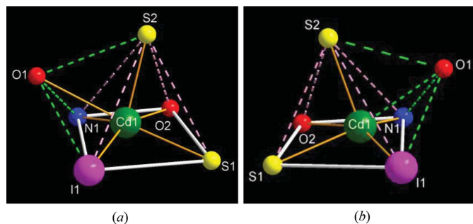
Figure 7 The coordination geometry of the cadmium(II) center in (a) 2 and (b) 3 , showing a distorted monocapped square-pyramidal arrangement.
