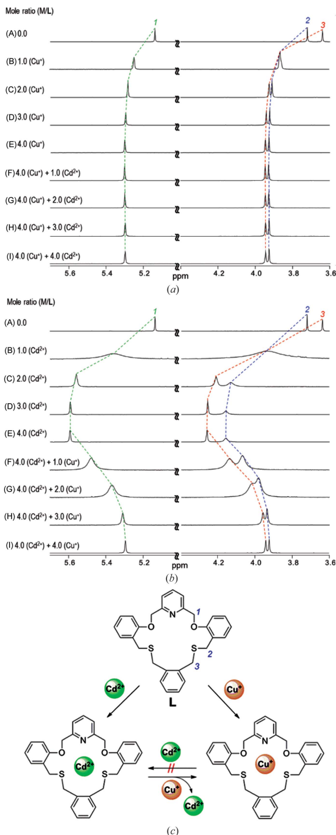
Figure 10 ^1\text{H} NMR spectra of the aliphatic region for L in \text{CD}_3\text{CN} via stepwise addition of (a) \text{Cd}^{2+} and \text{Cu}^+ , and (b) \text{Cu}^+ and \text{Cd}^{2+} . [ L ] = 5 mM. (c) The proposed complexation equilibria between the corresponding species in solution.
