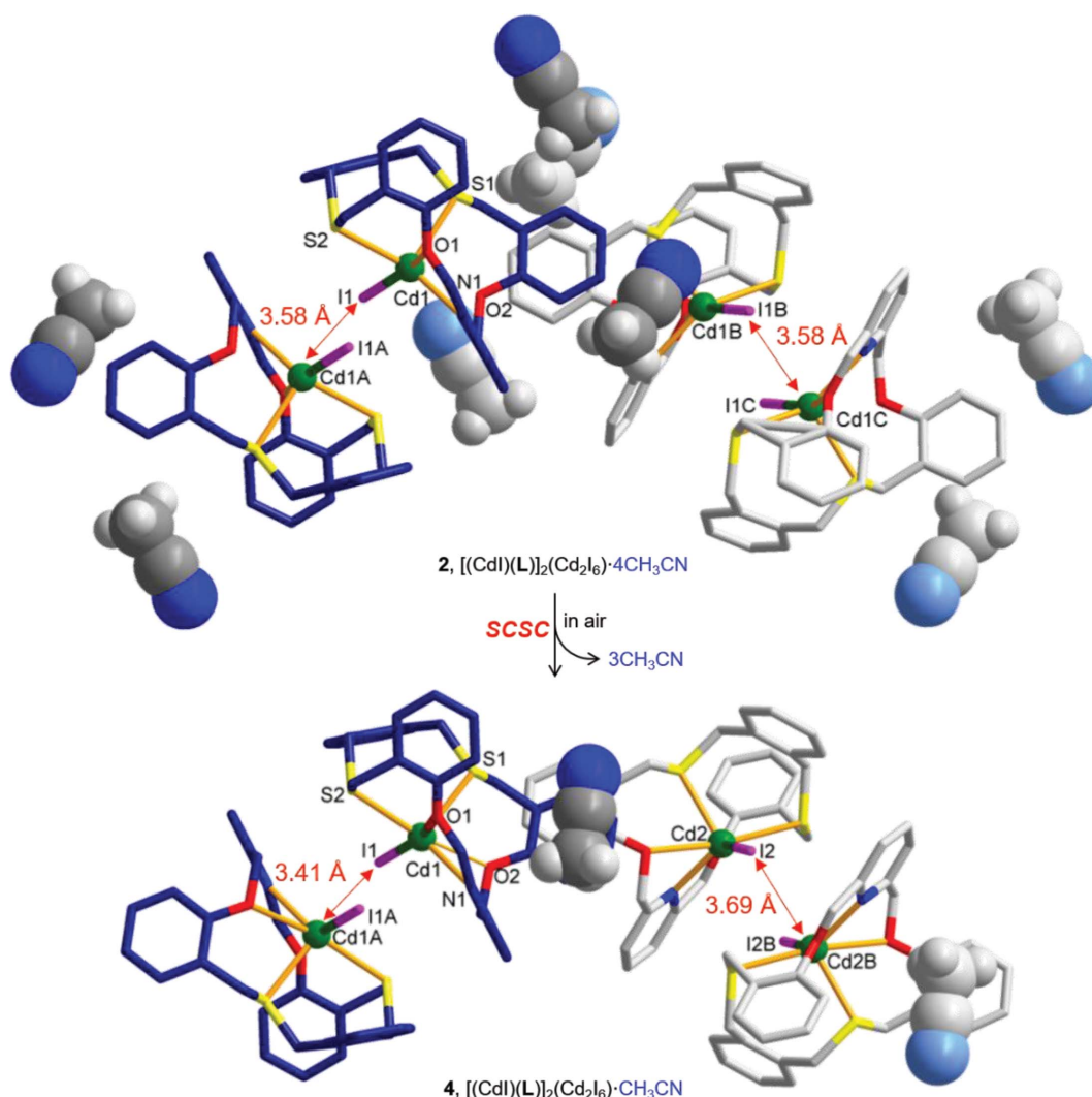
Figure 8 The SCSC transformation of 2 (top) to 4 (bottom) via the partial removal of the lattice solvent molecules. The anionic clusters (Cd 2 I 6 ) 2− have been omitted.
