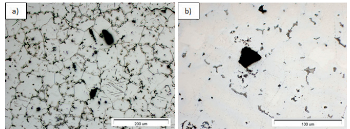
Fig. 1. Microstructure of the composites matrix, LM; a) grain structure of the WE43 alloy; b) eutectics morphology in the WE43 alloy
