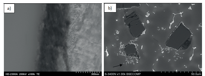
Fig. 5. Matrix/reinforcement interface structure; a) thin layer at the interface, STEM; b) layers of fine particles, SEM
