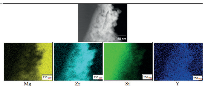
Fig. 6. Chemical composition of the SiC/WE43 interface
