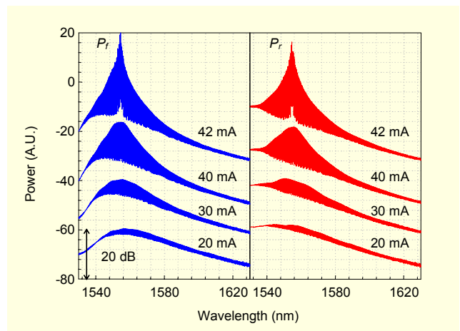
Fig. 3. ASE spectra at the front facet (left) and the rear (right) for the integrated LD ( w_d=3.5 \mu\text{m} ) at currents of 20, 30, 40, and 42 mA.
