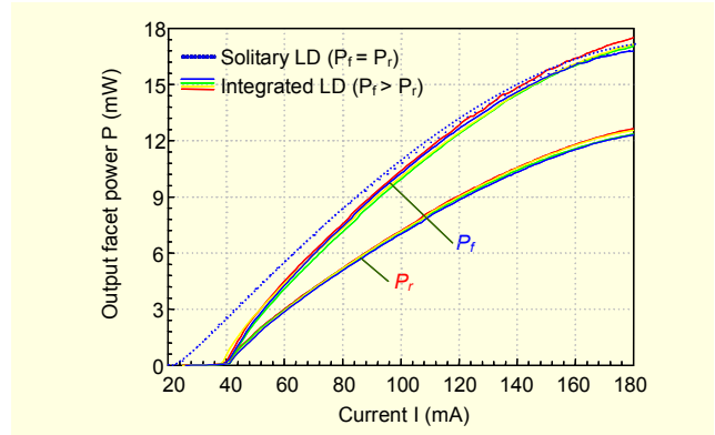
Fig. 2. P - I characteristics of a 600 \mu\text{m} long solitary LD (dotted line) and integrated LDs with w_d=3, 3.5, 4, 4.5 \mu\text{m} , L_s=600 \mu\text{m} , and L_d=400 \mu\text{m} (solid lines) under CW operation (22°C).
